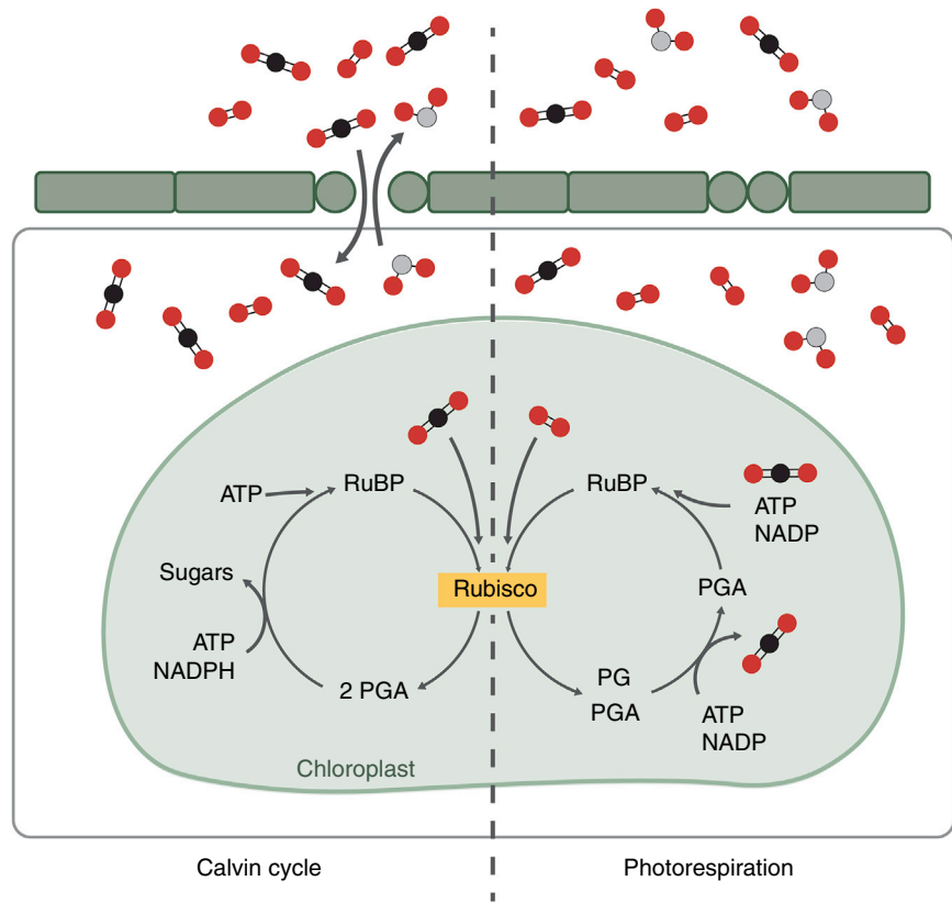
Figure 1. Calvin cycle and photorespiration in response to drought showing the enzyme Rubisco's carboxylase and oxygenase activities.
