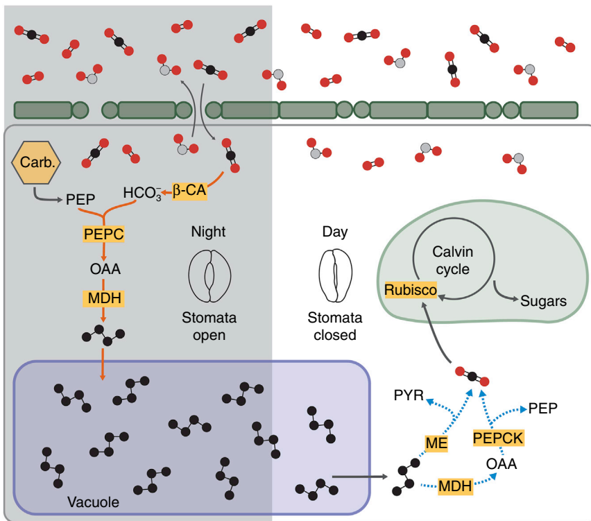
Figure 2. Crassulacean acid metabolism.
