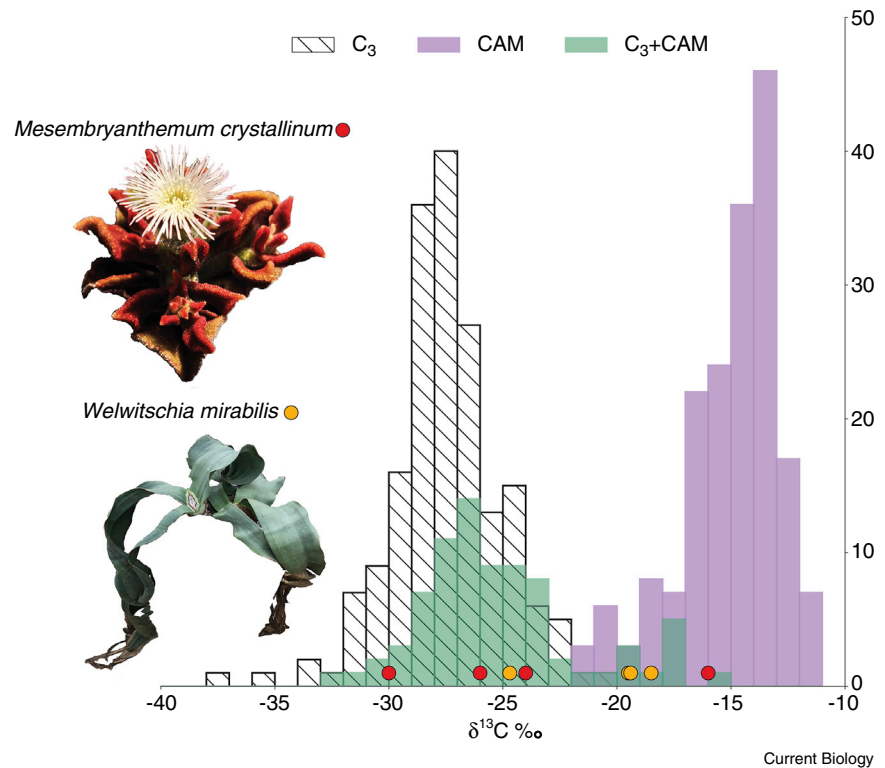
Figure 3. Distribution of carbon isotope ratios from 385 species from 19 clades of lycophytes, ferns, gnetophytes, monocots, and eudicots.
